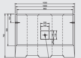
M20 Short Wavy Tailed Lifting Socket 2000Kg SWL
