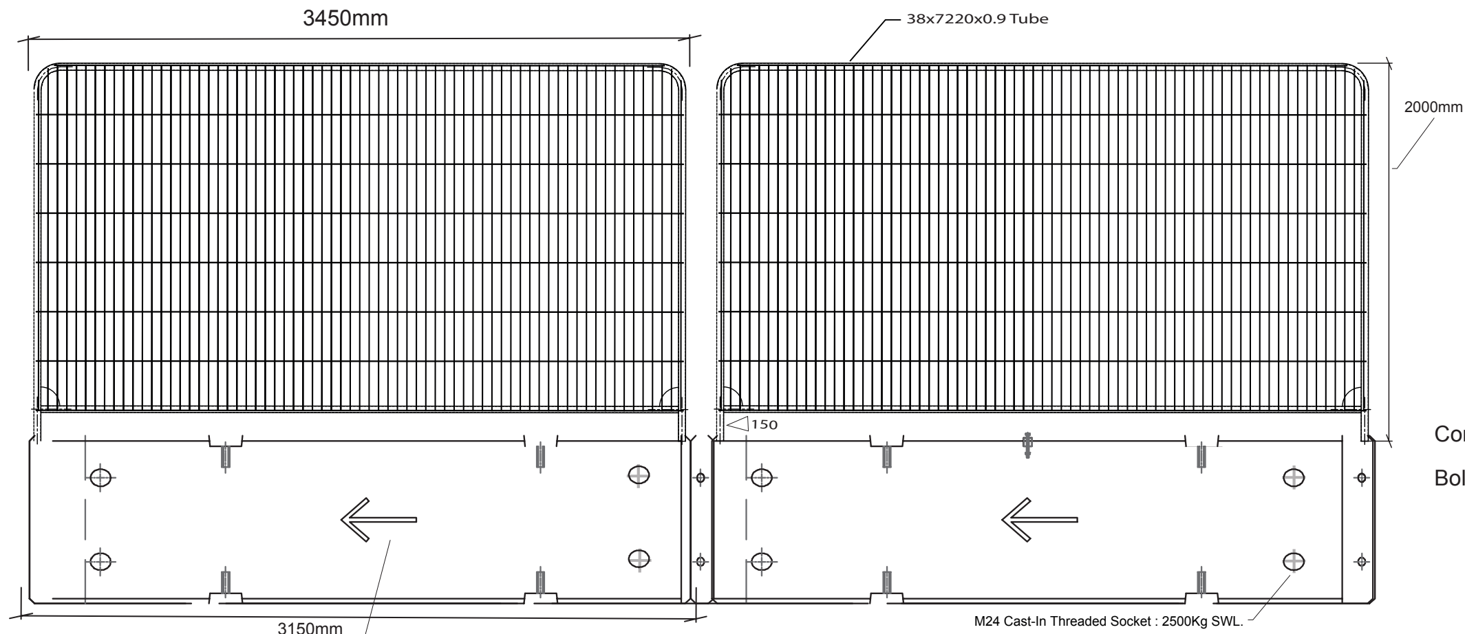
FRONT VIEW (FROM DIRTY SIDE)
